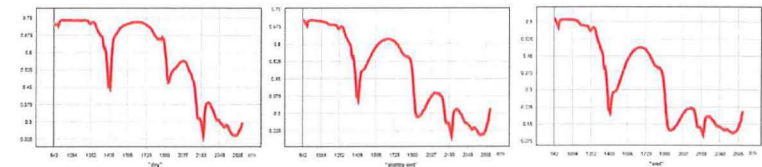
Figure 20.7: Average spectra of the measured area in Fig. 20.6 at different moisture contents on the sample surface [8].
